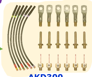
AKD300 3x120A cables with terminals
